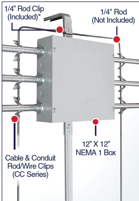
Shown with Enclosure Installation (Front)
