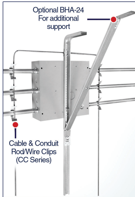
Shown with Enclosure Installation (Back)
