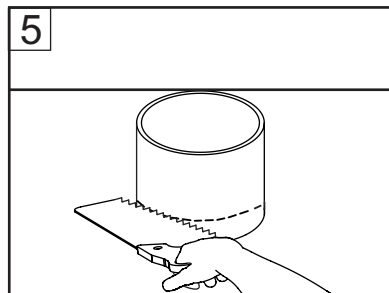
Using line as a guideline, cut excess material with saw.
