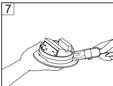
Apply solvent cement to PVC Adapter Ring.
