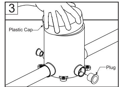
Install plastic cap and seal unused outlets. Apply concrete.
