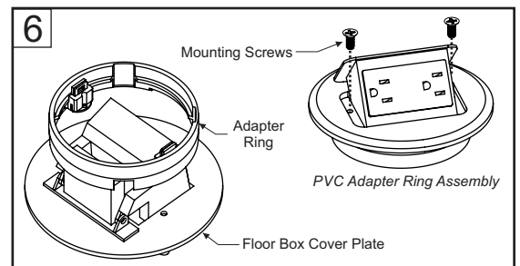
Install PVC Adapter Ring to desired round floor box cover.
