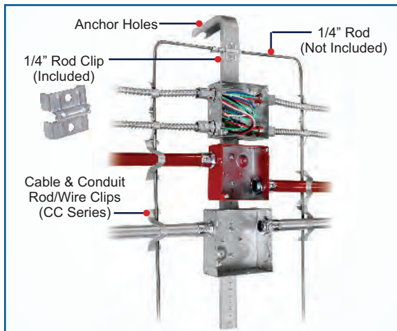
Shown with Multi-System Installation
