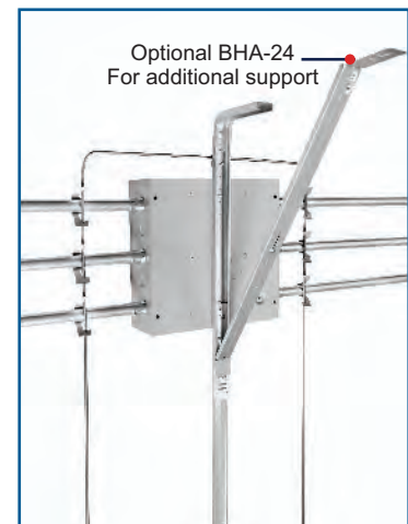
Shown with Enclosure Installation (Front & Back)
