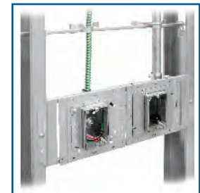
SSR-16 & CC Clips provide MC & Conduit Support
