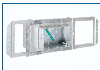
Break UMA in half to mount Multigang Boxes
