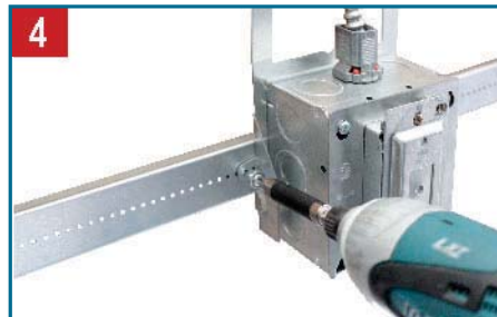
Secure the assembly to the BHA with Tek screws, setting the box in place
