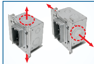
Turn any 4", 4-11/16" and 5" sq. box 90° with UMA-LVBS
