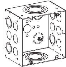
T5B-50/200 5" x 5" x 3-1/4"
